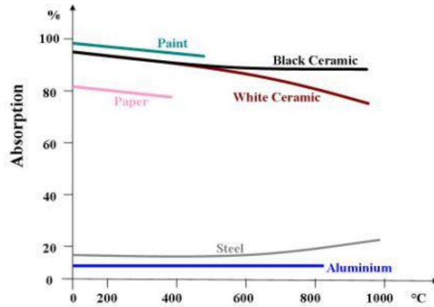
Figure 5: Absorption of various materials
