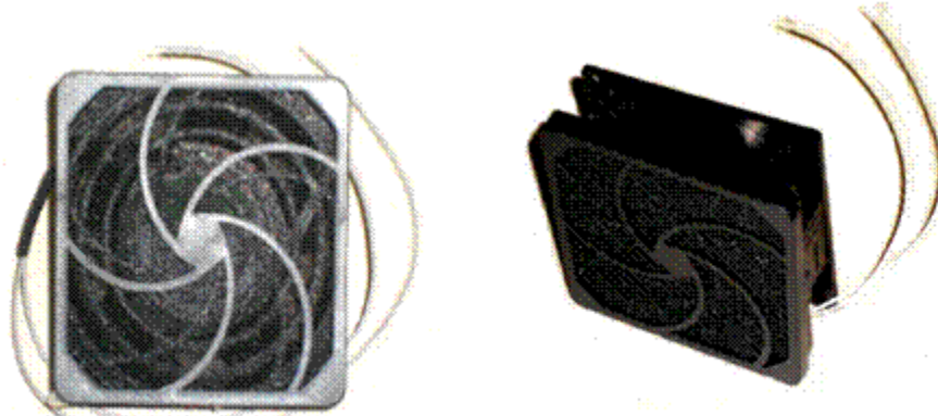
Front View: 3.625" x 3.625" x 1.437" T Angle View: 3.625" x 3.625" 1.437" T
