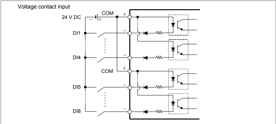
Circuit configuration of digital input
