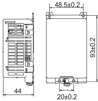
(Panel mounting hole dimensions)
