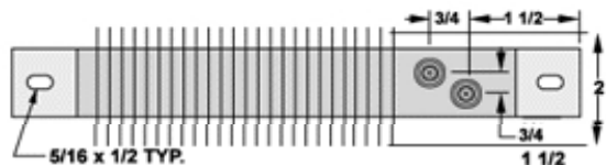
TYPE 4 Termination
