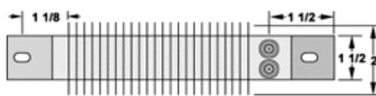
TYPE 2 Termination
