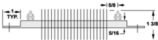
TYPE 1 Termination
