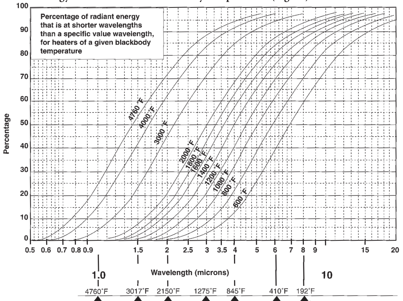
Source Temperatures (°F) For The Peak Radiation Band's Wavelength (Wien's Displacement Law)
