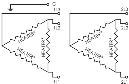
TWO THREE-PHASE DELTA CIRCUITS
