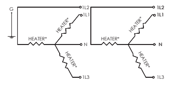
TWO THREE-PHASE WYE CIRCUITS
