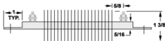
TYPE 1 Termination
