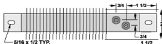
TYPE 4 Termination
